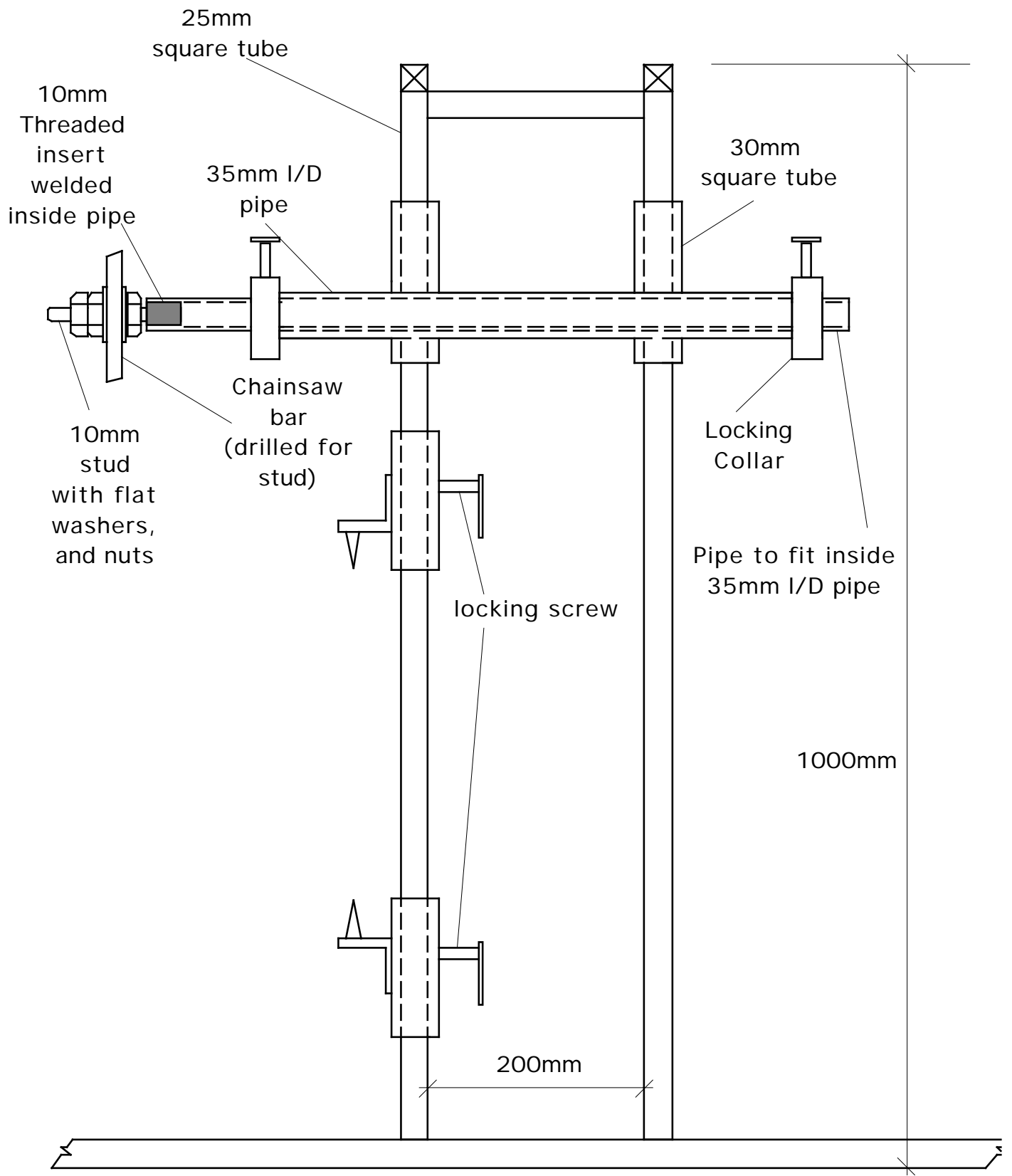
Side View
