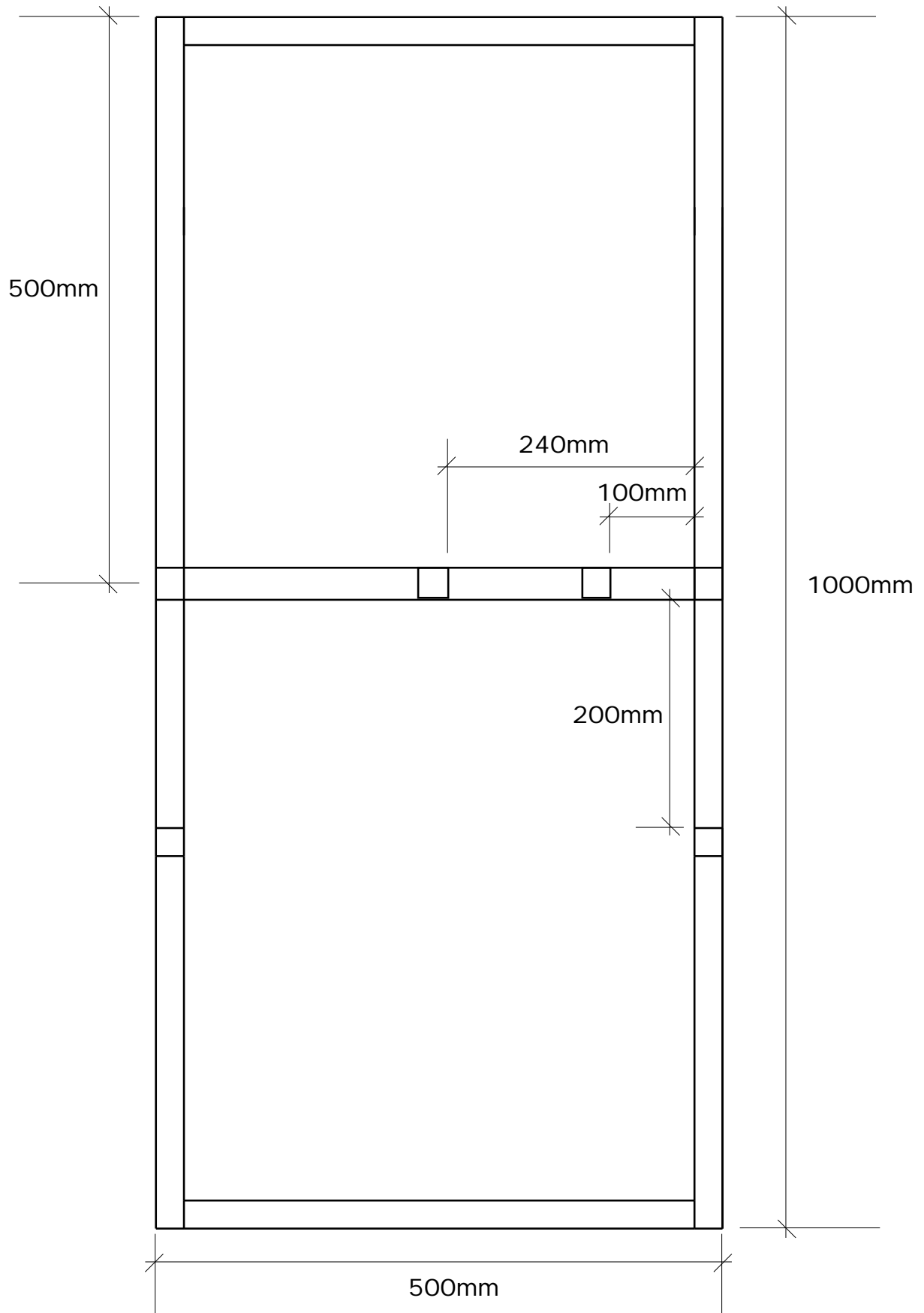
Plan View
