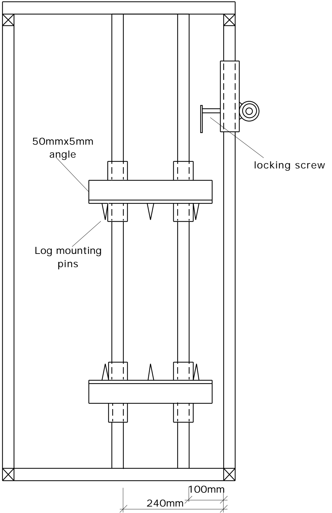
Front View
